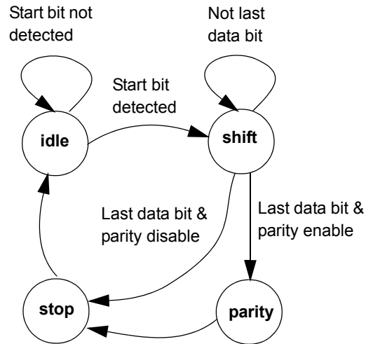
Figure 2: Receiver State Machine
