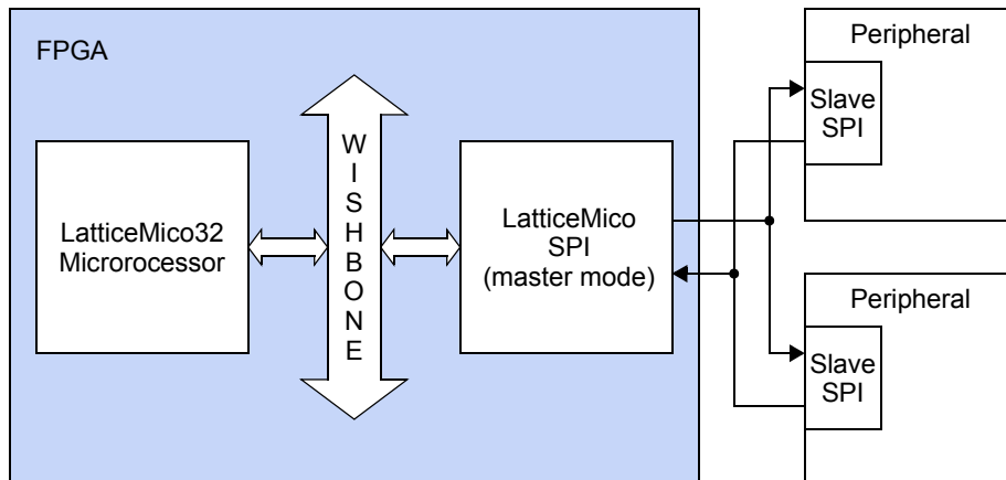
Figure 1: Using LatticeMico SPI to Communicate with Peripherals
