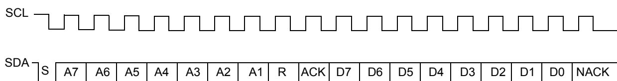
Figure 4: Single-Byte Read Waveform
