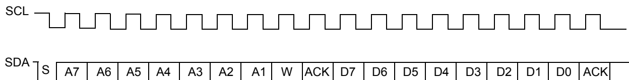
Figure 3: Single-Byte Write Waveform
