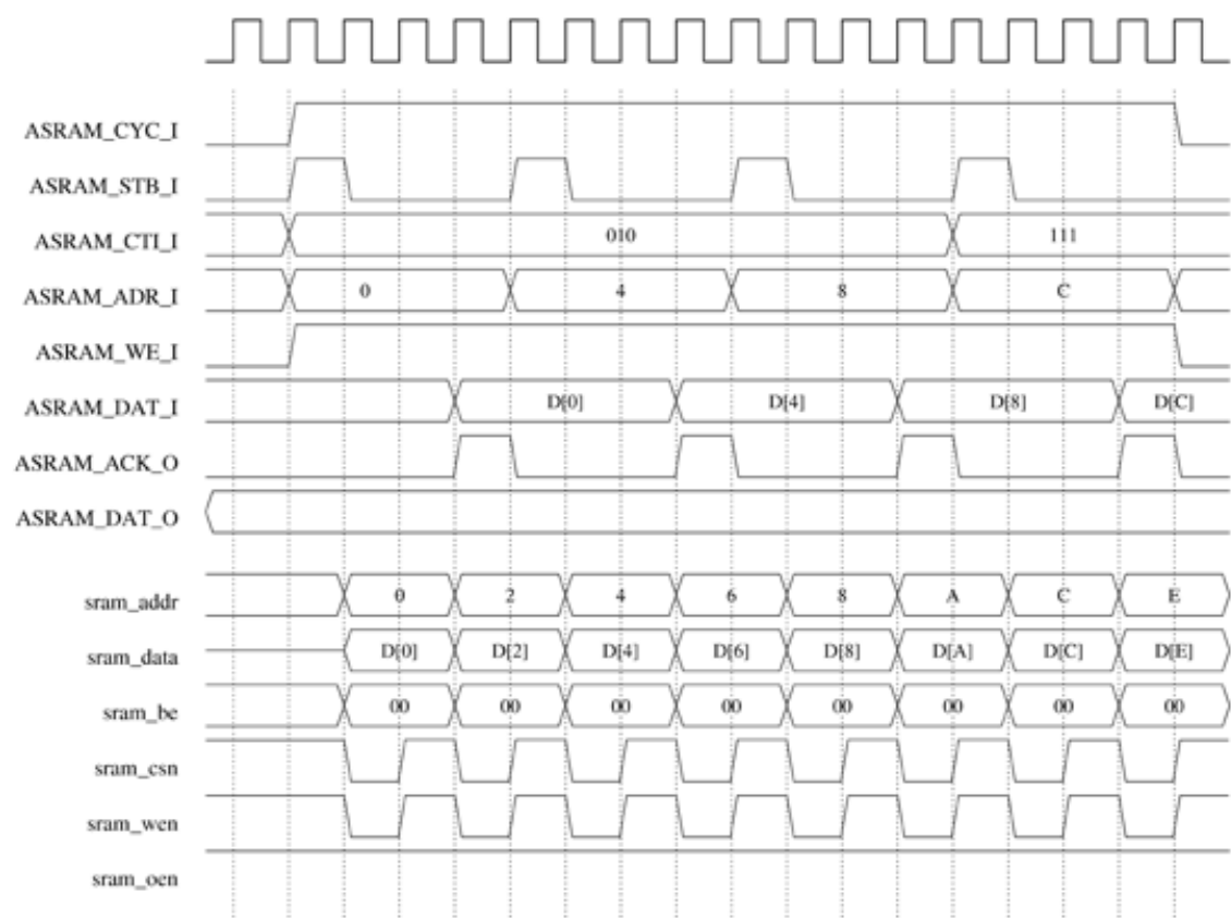
Figure 7: WISHBONE 32-Bit Burst Write (Asynchronous SRAM with 16-Bit Data Bus)
