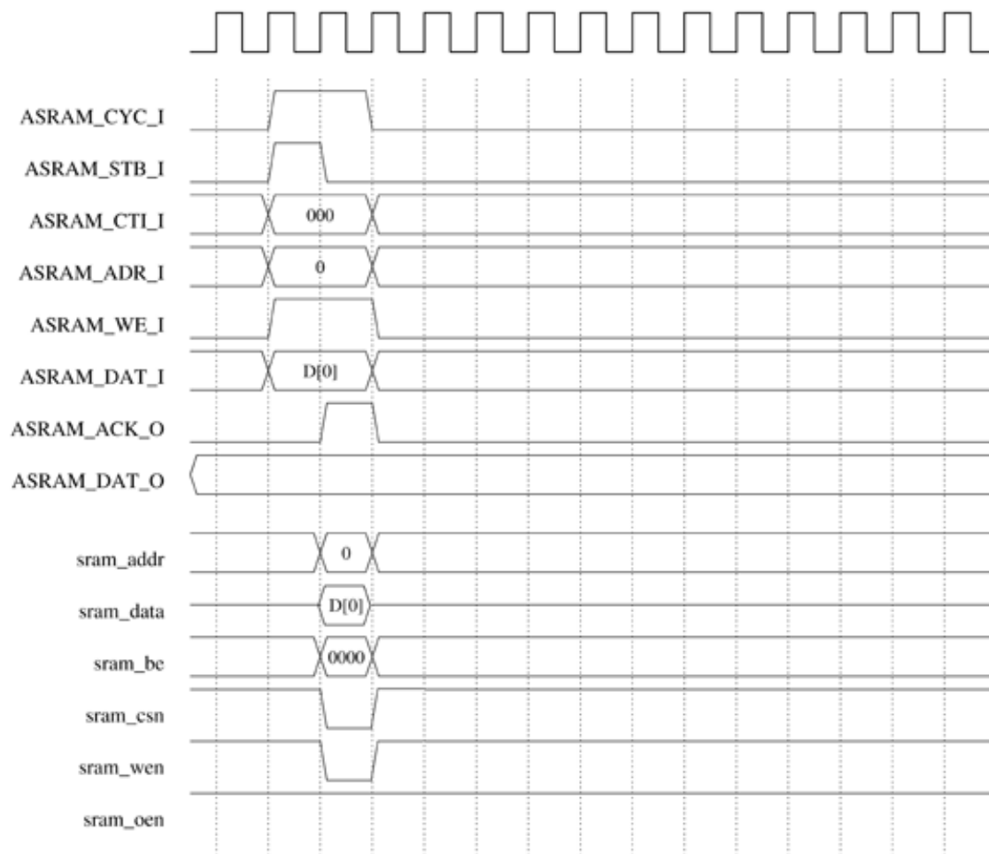
Figure 4: WISHBONE 32-Bit Classic Write
