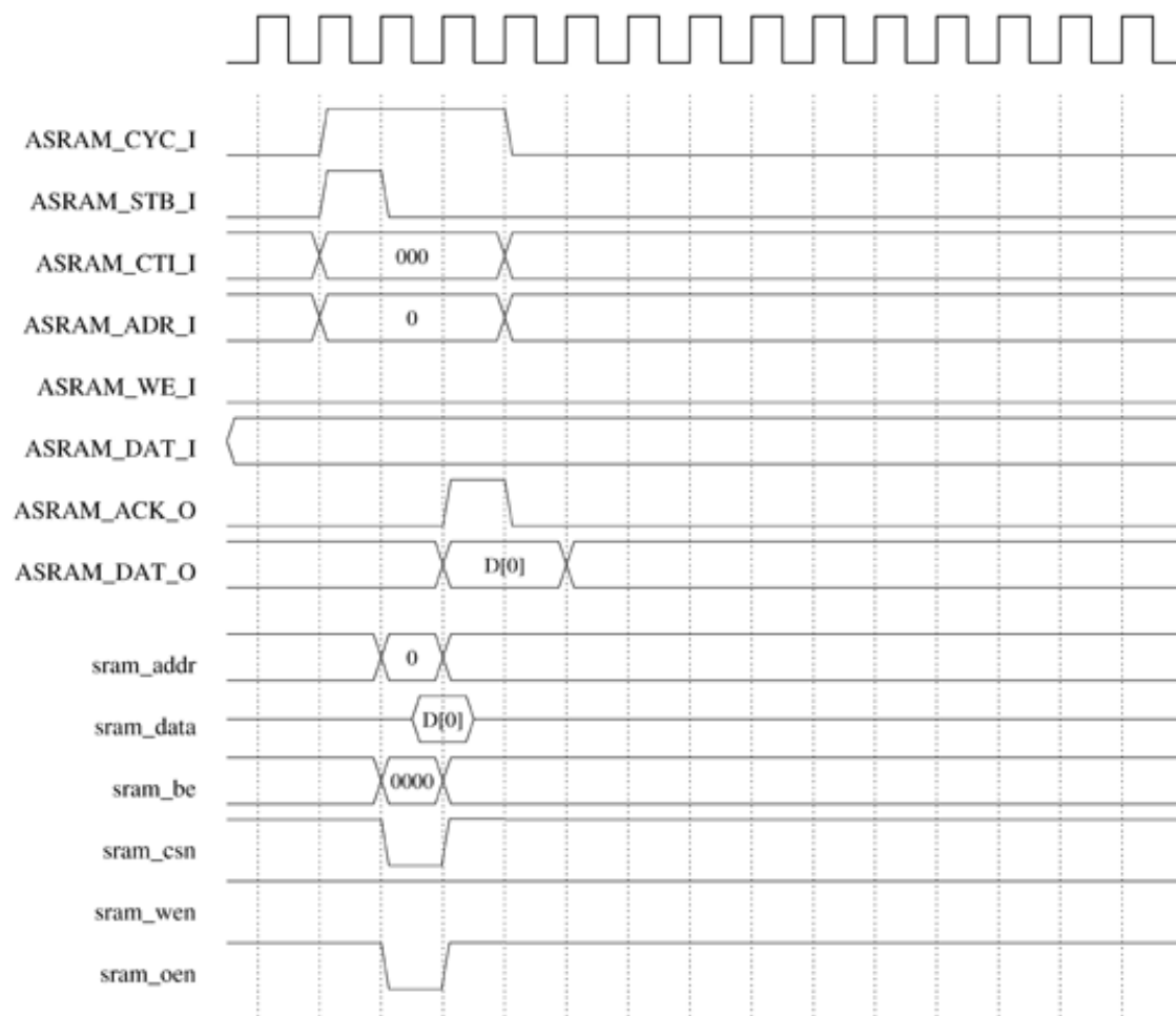
Figure 3: WISHBONE 32-Bit Classic Read (registered read)
