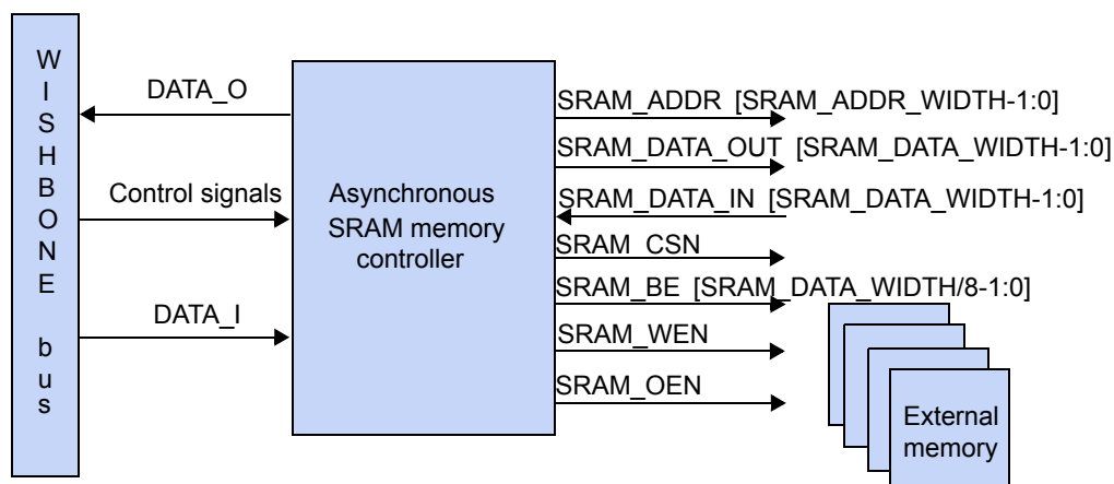
Figure 1: Asynchronous SRAM Usage
