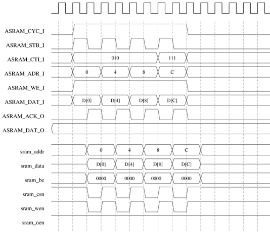
Figure 6: WISHBONE 32-Bit Burst Write
