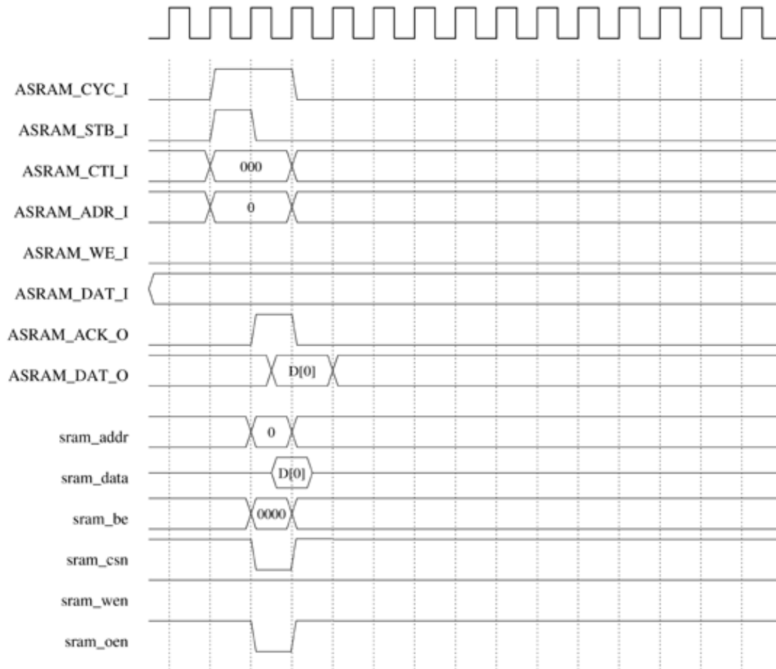
Figure 2: WISHBONE 32-Bit Classic Read (non-registered read)
