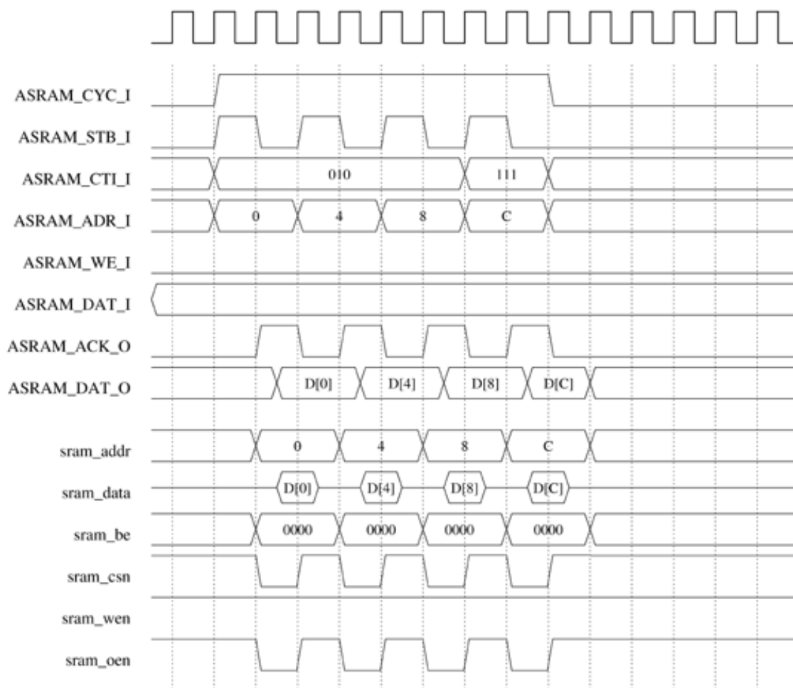
Figure 5: WISHBONE 32-Bit Burst Read (non-registered read)
