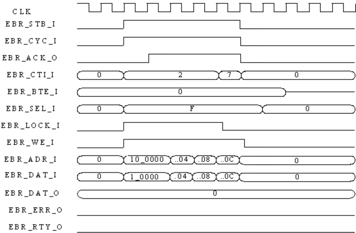
Figure 4: On-Chip Memory Controller Timing Diagram for Burst 4 Write Mode
