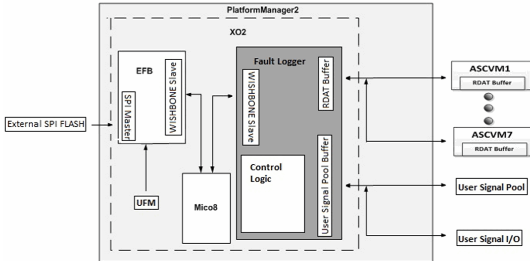
Figure 1: Fault Logger Block Diagram
