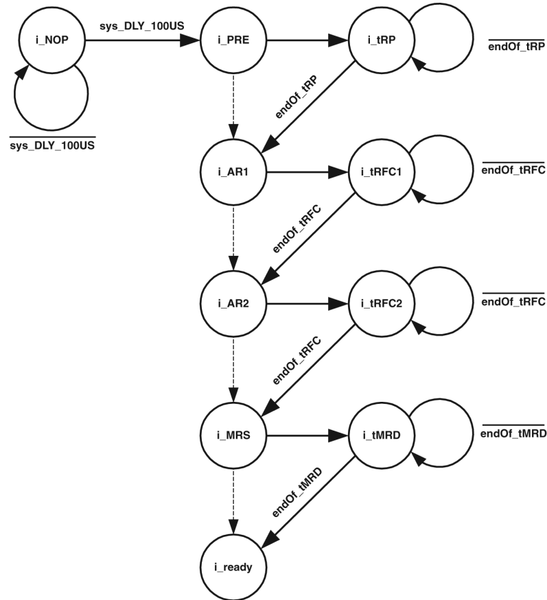
Figure 4: INIT_SFM State Diagram
