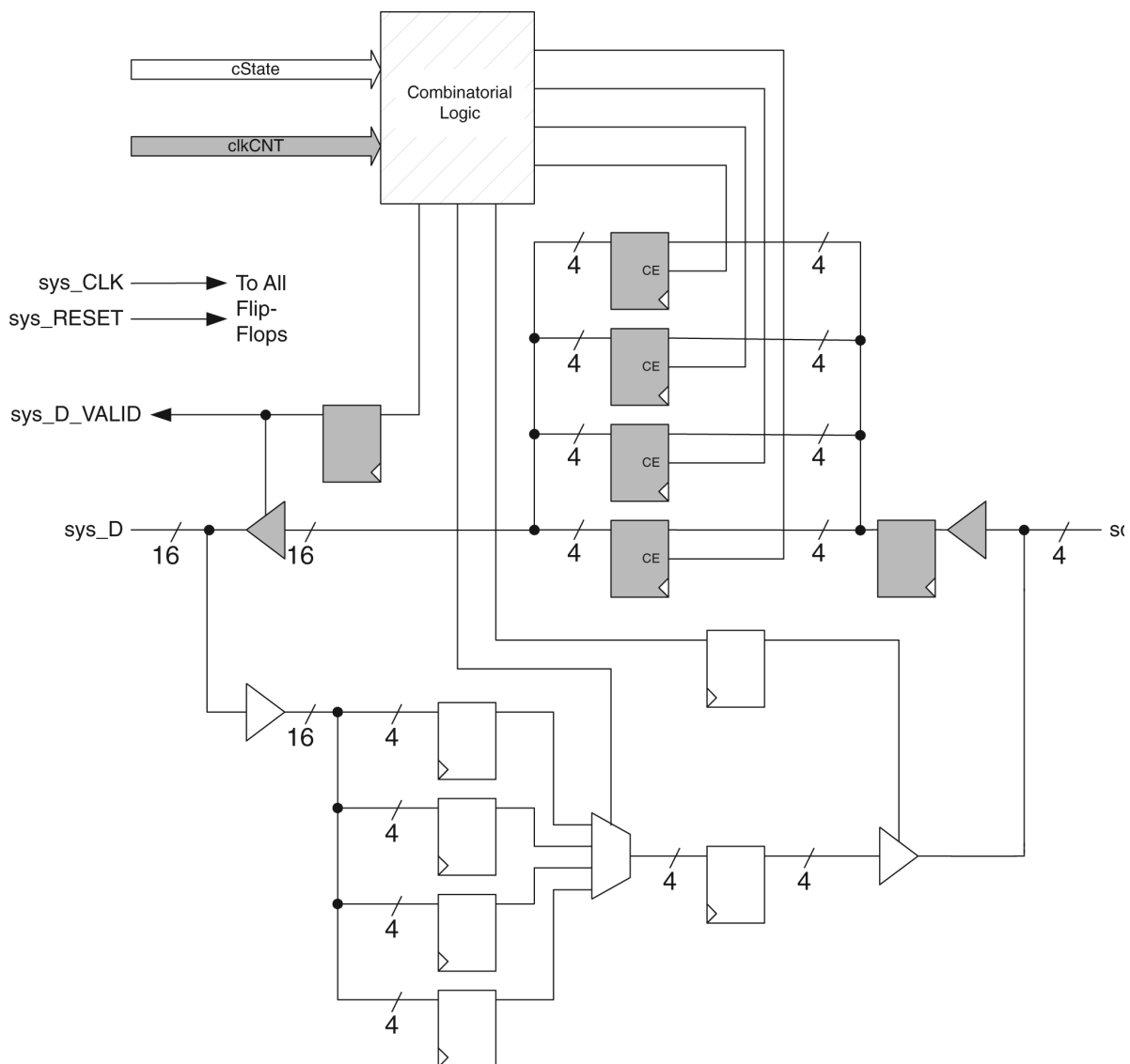
Figure 6: Data Path Module
