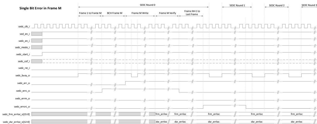
Figure 6.5. SEDC Continuous Mode with Correctable Error (sedc_cof_i = 0/1)
