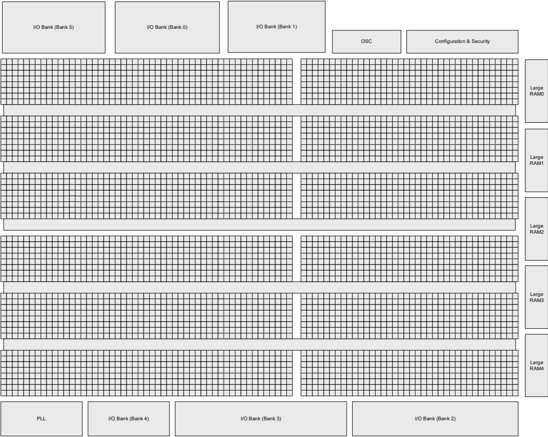
Figure 2.1. LIFCL-33 Simplified Block Diagram
