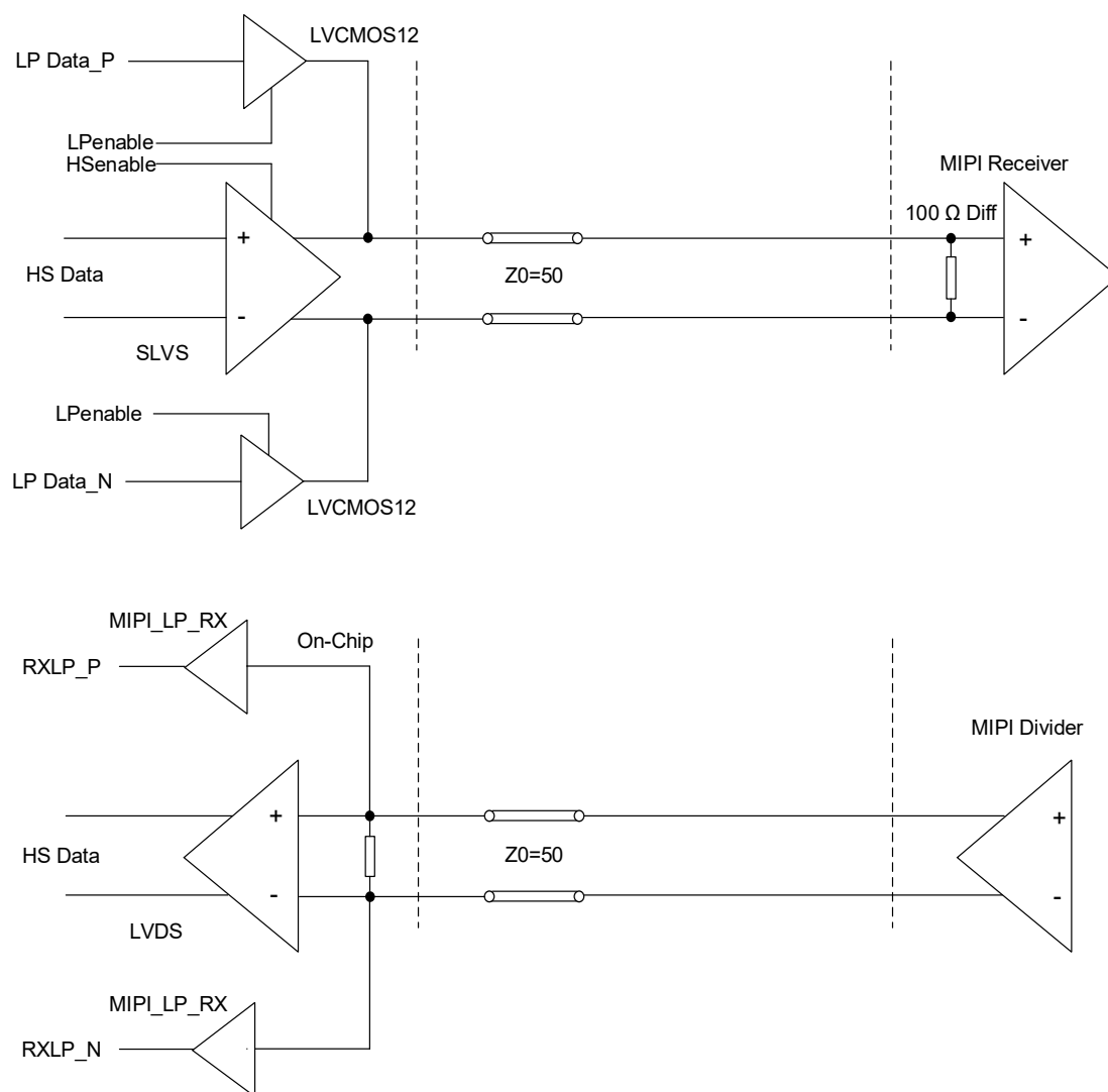
Figure 3.6. MIPI Interface
