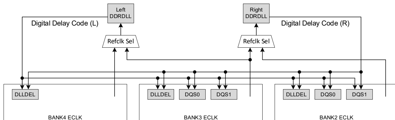
Figure 2.12. DDRDLL Architecture
