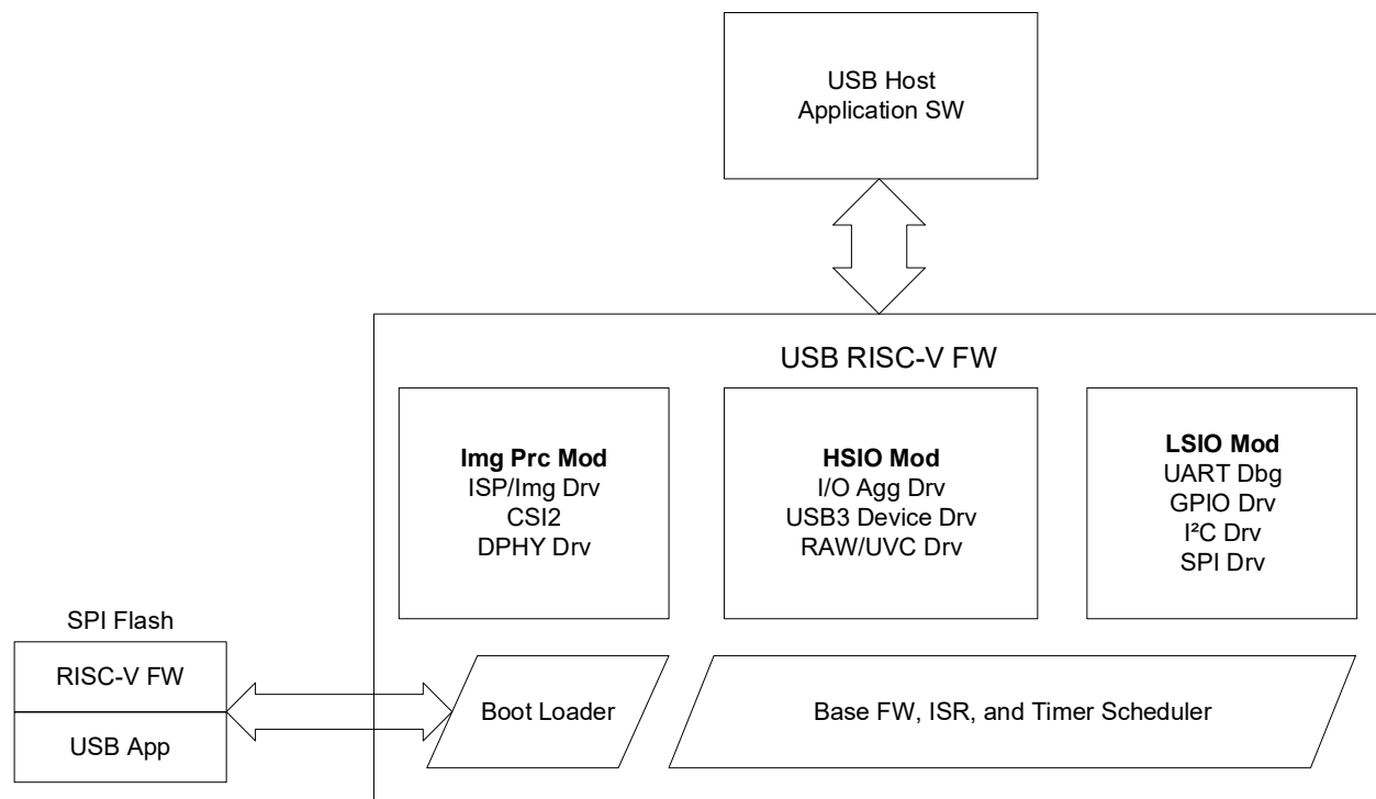
Figure 2.26. LIFCL-33U USB RISC-V Host FW Stack
