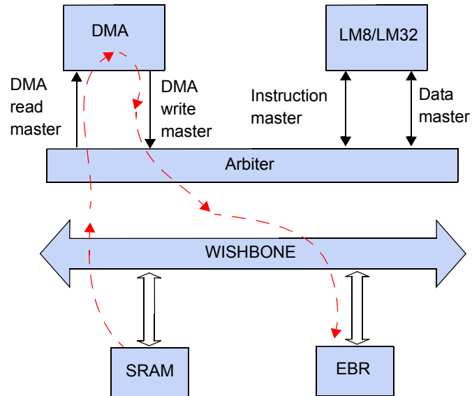
Figure 1: DMA Usage with Shared-Bus Arbitration in LatticeMico System
